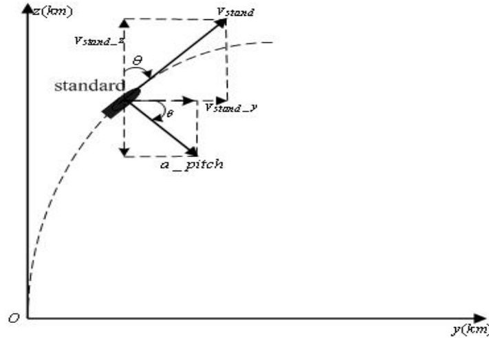
Figure 2 Vertical Acceleration Stage Model of Standard-2 Missile
